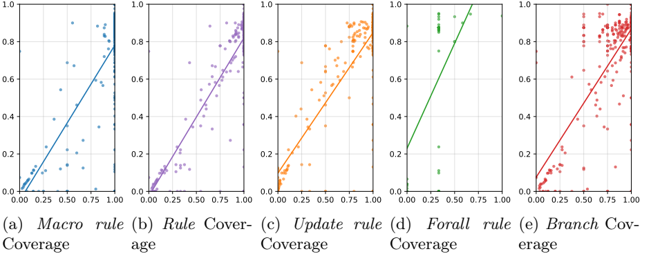
Fig. 5: Coverage Criteria vs. Mutation Score for Avalla scenarios on Asmeta specifications
