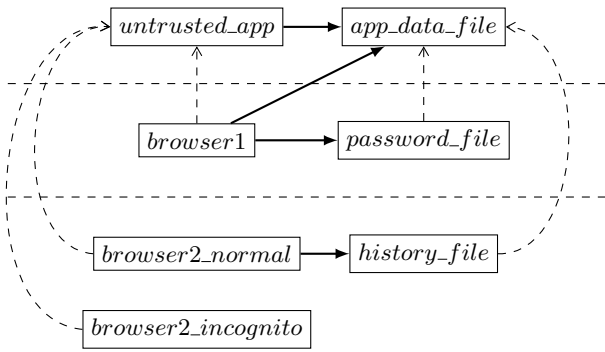
Figure 7: Isolation of two applications using typebounds.
