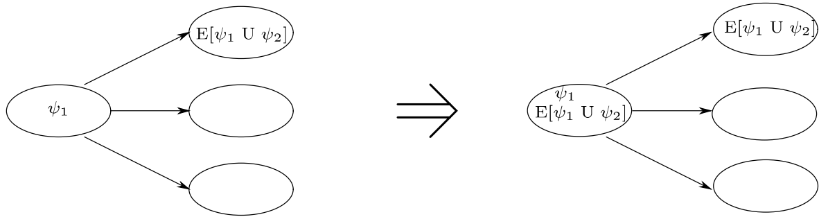
Figure 3.25. The iteration step of the procedure for labelling states with subformulas of the form E[\psi_1 \text{ U } \psi_2] .
