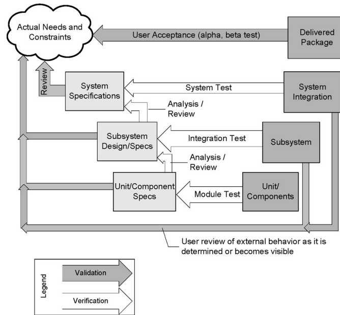
Figure 1.2: Validation activities check work products against actual user requirements, while verification activities check consistency of work products.
