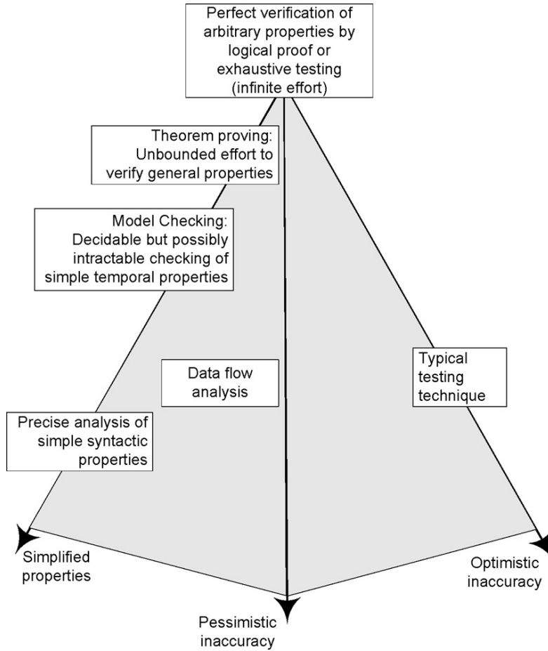
Figure 1.3: Verification trade-off dimensions
