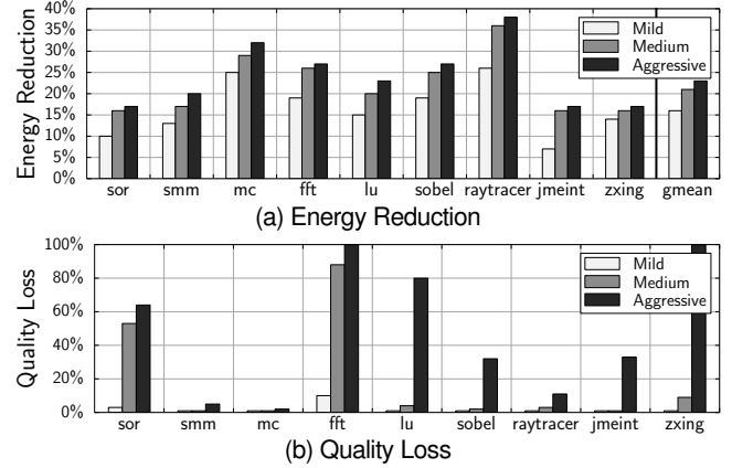
Figure 10: (a) Energy reduction and (b) quality loss when approximating all the safe-to-approximate data and operations.
