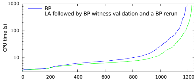
Figure 7: Quantile plot showing that LA followed by a BP witness validation and rerunning BP on rejections is more efficient and effective than just running BP
