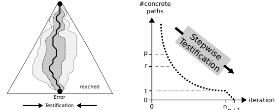
Figure 2: Testification reduces the state space (left) and the number of paths (right) that need to be (re-)verified.
