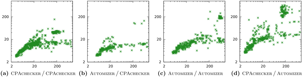
Figure 5: Scatter plots for pairwise composition for witness validation: CPU seconds for producing a witness on the x axis, CPU seconds for witness validation on the y axis. A caption “ p/c ” abbreviates “witnesses produced by p that are accepted by c ”
