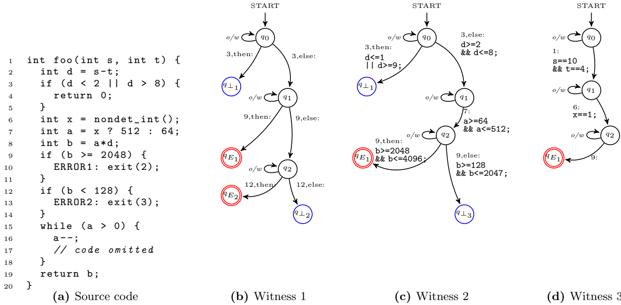
Figure 3: Example C program (a) and a testification sequence of three witness automata: accepting control states are drawn as double circles, sink states are labeled with the subscript \perp , non-accepting control states are drawn as single circle.
