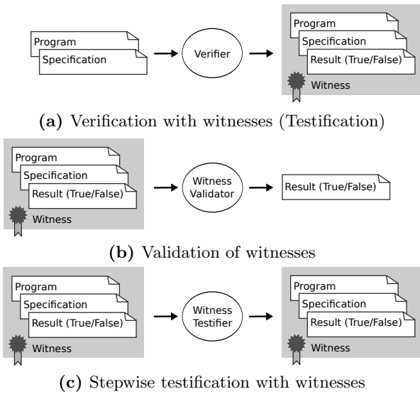
Figure 4: From verification and witness validation to stepwise testification
