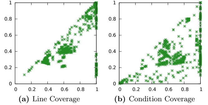
Figure 6: Scatter plots that illustrate a reduction of the code coverage with values for the verification runs on the x axes and values for the witness-validation runs on the y axes
