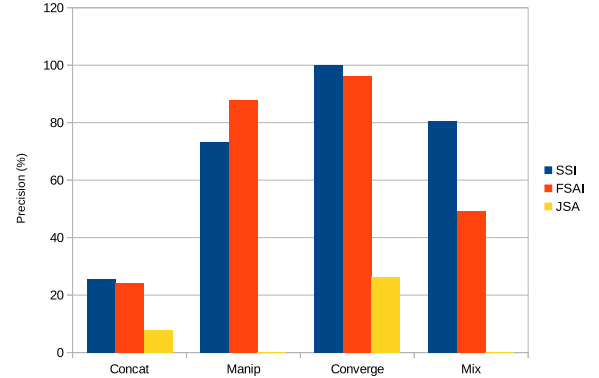
Figure 2: Precision of the three analyses on varied data flows.
