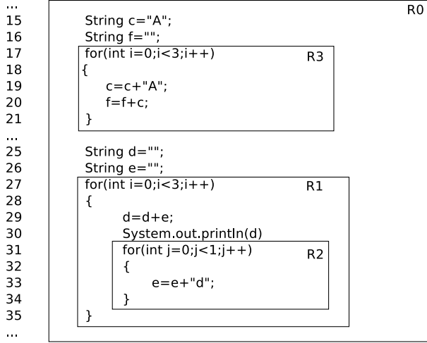
Figure 1: The Region Tree for Program 1
