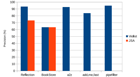
Figure 3: The precision of market apps
