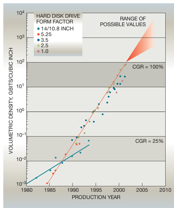
Figure 4 Hard disk drive volumetric density trend
